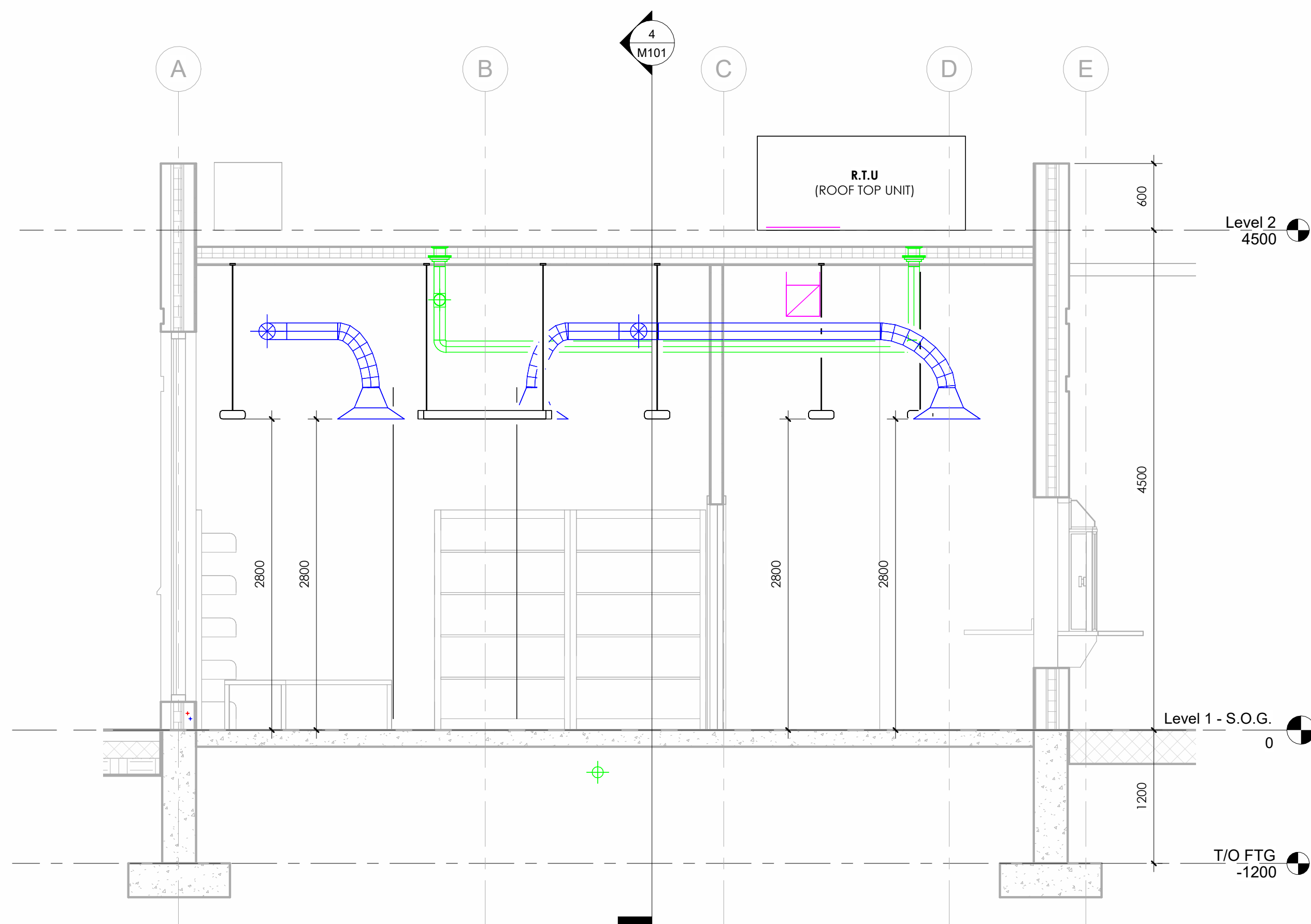
SYSTEMS M.E.P. SECTION 1
