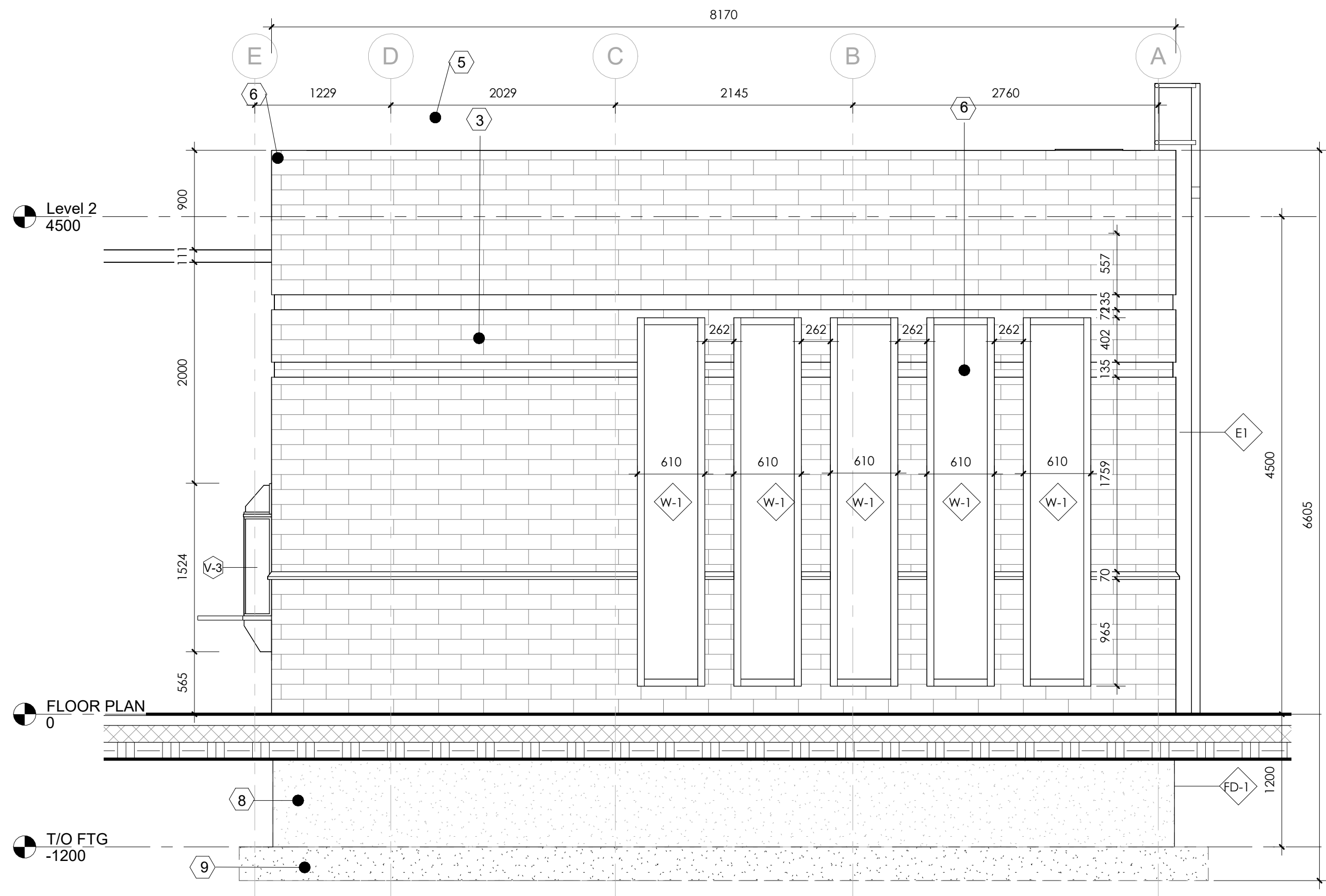
1 NORTH ELEVATION 3/8" = 1'-0"
