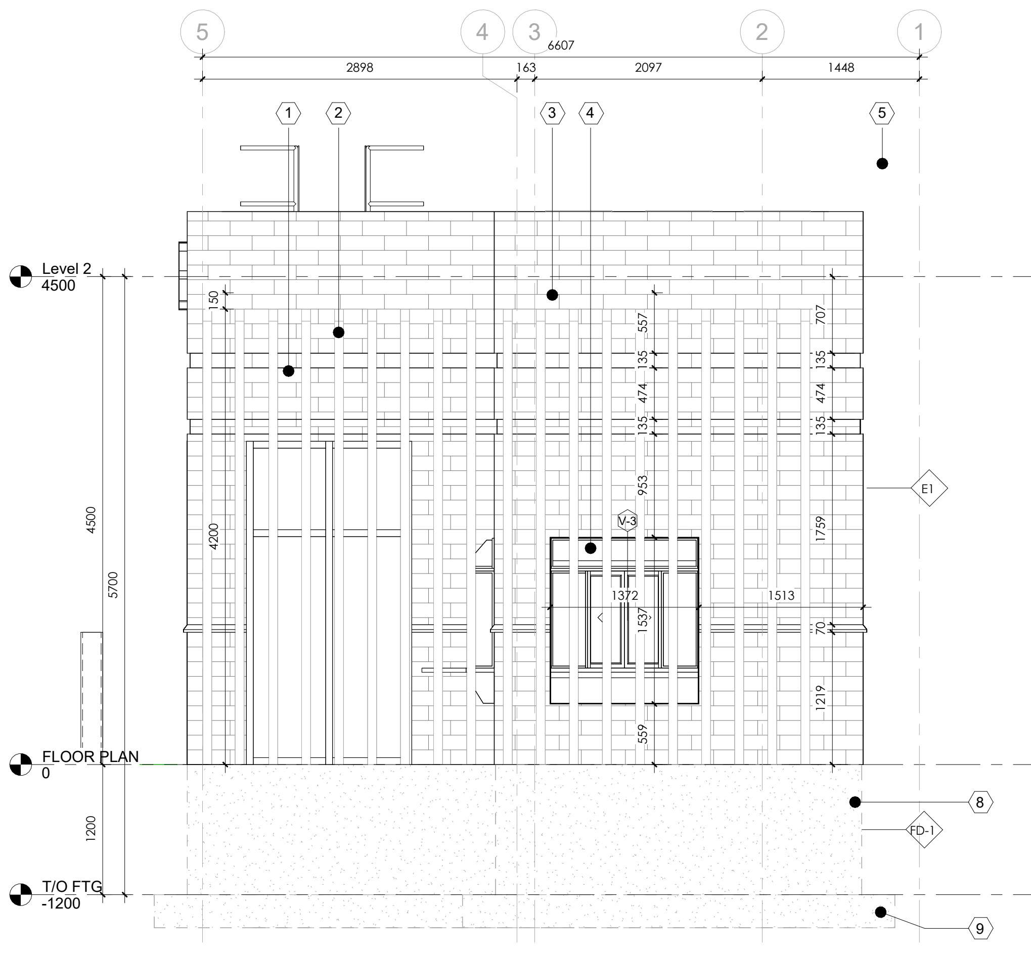
EAST ELEVATION 3/8" = 1'-0"
