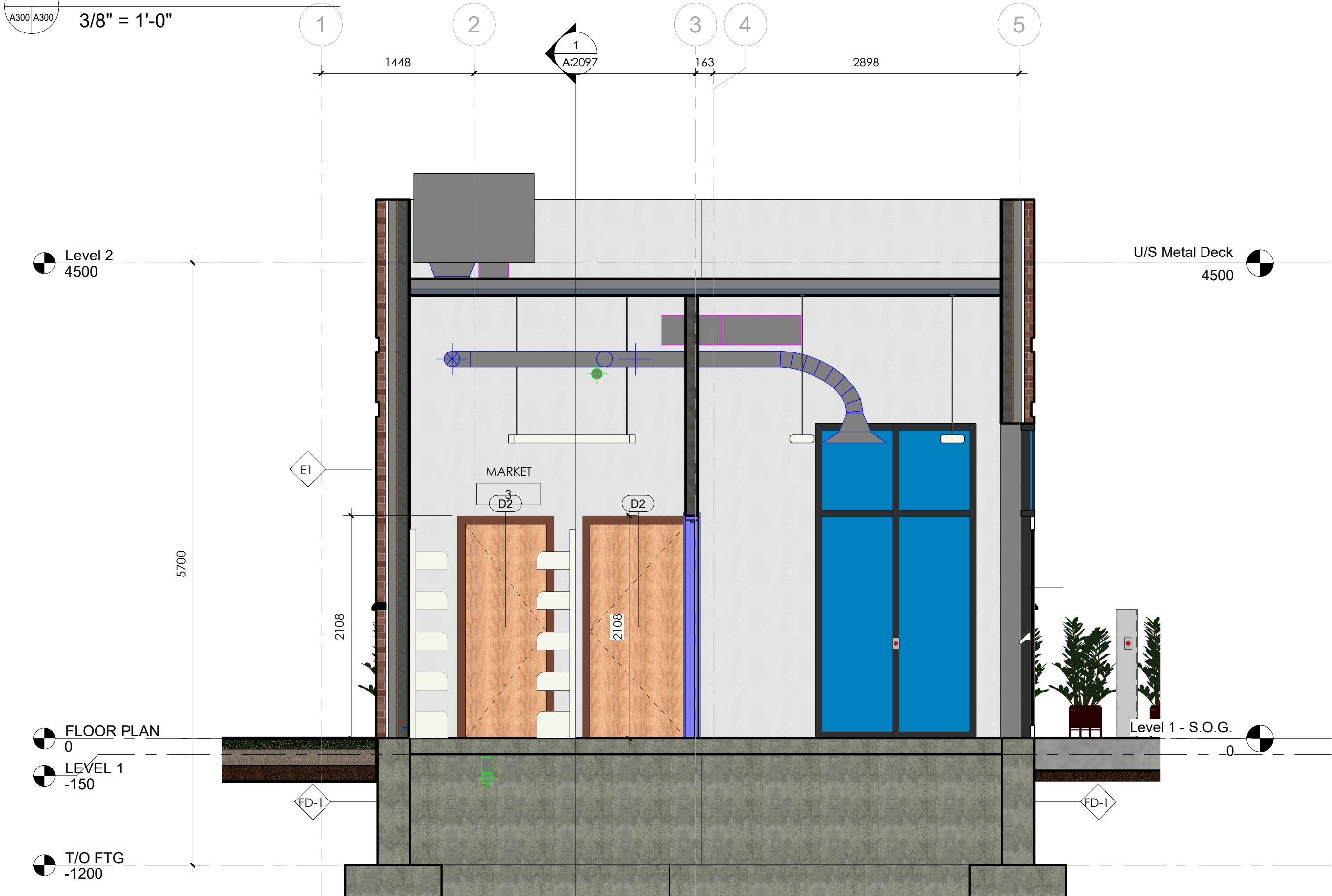
BUILDING SECTION 2 3/8" = 1'-0"
