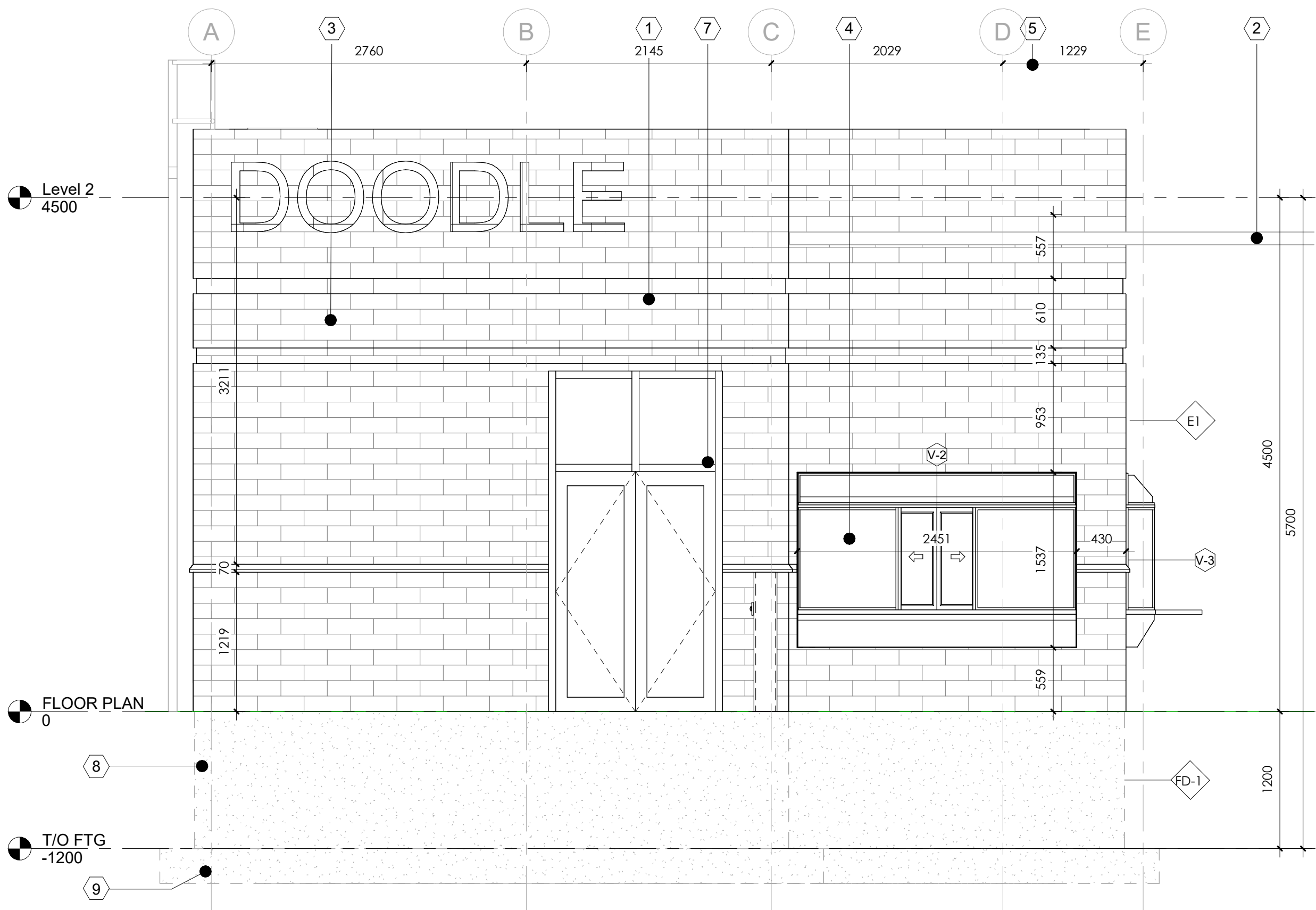
SOUTH ELEVATION 3/8" = 1'-0"
