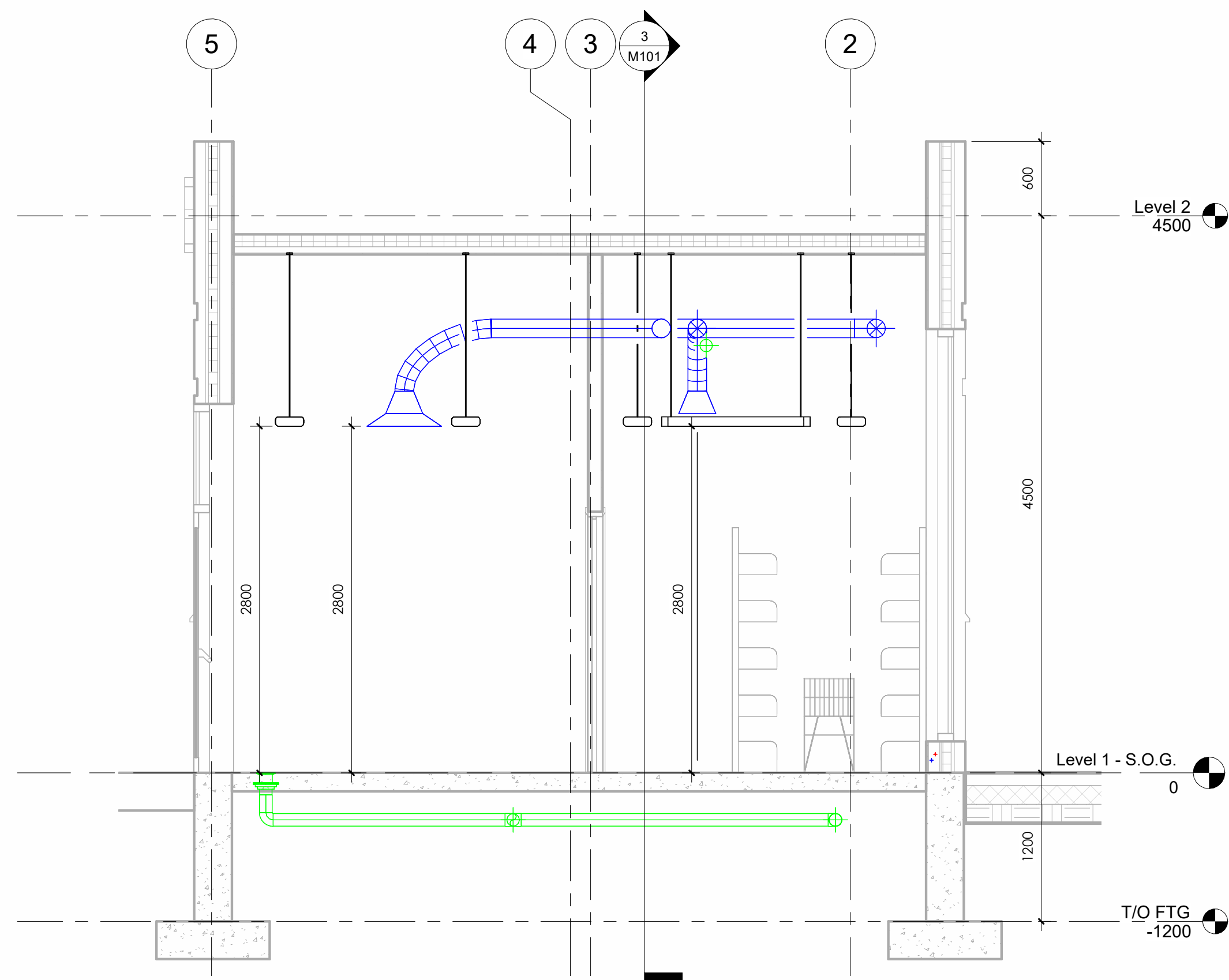
SYSTEMS M.E.P. SECTION 2
