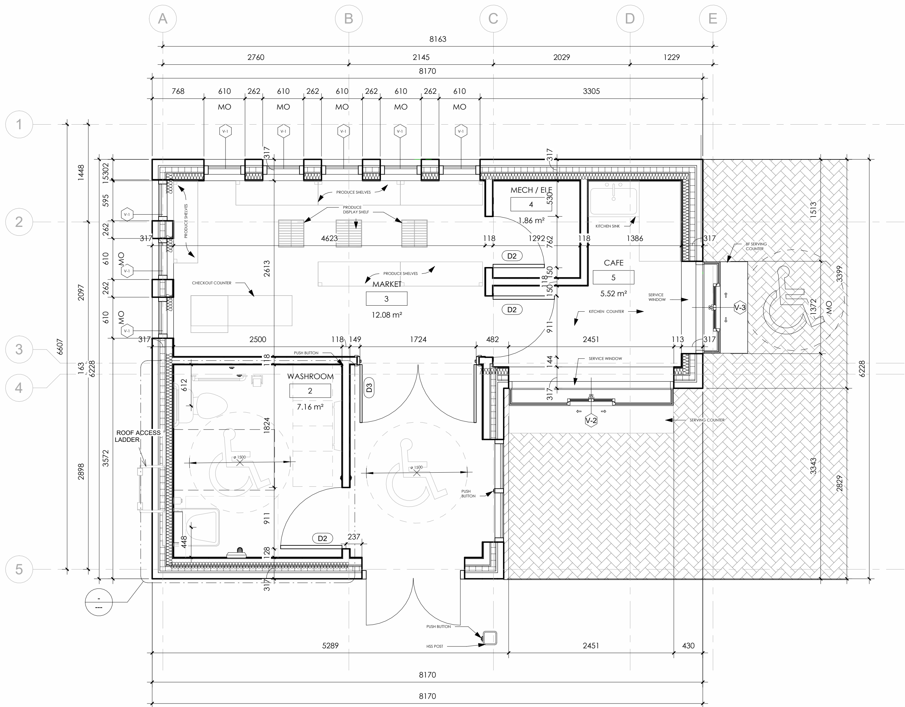
1 FLOOR PLAN 3/8" = 1'-0"
