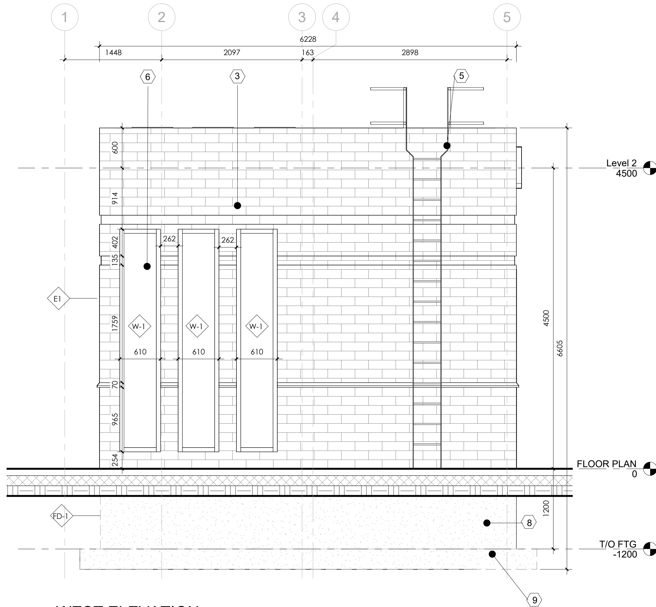
2 WEST ELEVATION 3/8" = 1'-0"
